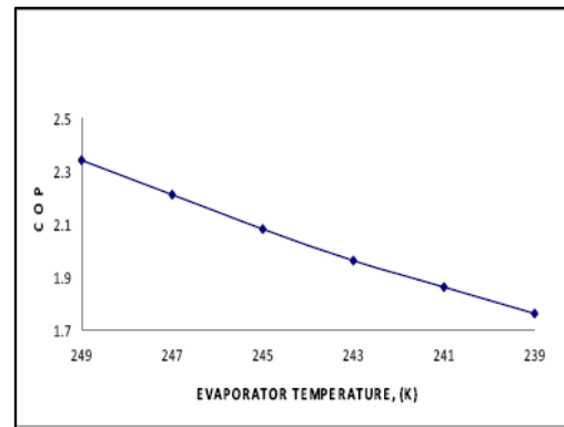
Fig: 12. Plot between the COP vs. Evaporator Temperature
