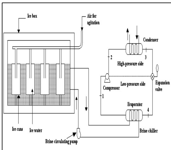
Fig: 1a. Schematic Diagram of an Industrial Ice Plant
