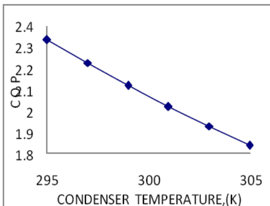
Fig: 11. Plot between the COP vs. Condenser Temperature
