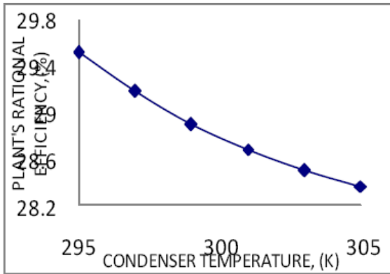
Fig: 9. Plant's Rational Efficiency Dependence upon the Condenser Temperature
