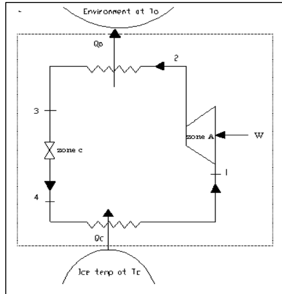
Fig: 1a. Schematic Diagram of an Industrial Ice Plant
