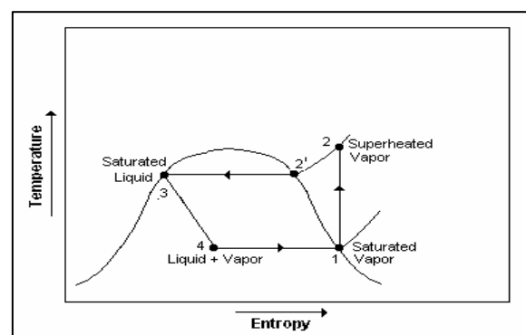
Fig: 2. T-s Diagram of Single Stage Vapour Compression Cycle
